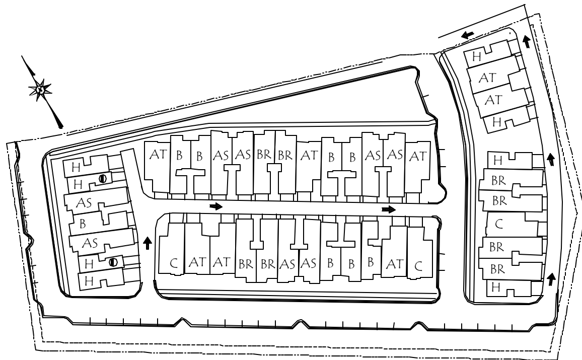
PRELIMINARY SITE PLAN - 43 UNITS
