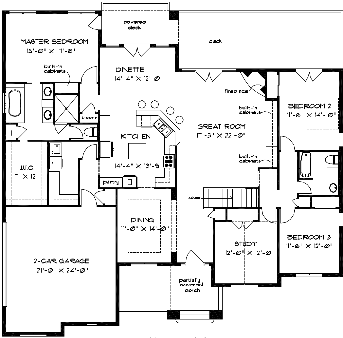
FLOOR PLAN 2,478 sq. ft.
